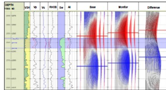
Figure 2: 4D Fluid substitution and offset synthetic modeling
