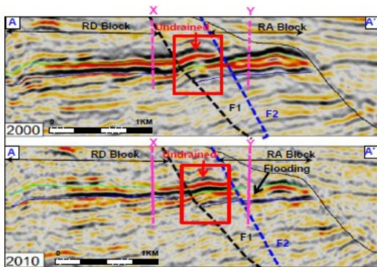
Figure 7: 4D sections reveal the impact of an intra-block fault on fluid flow and shows a potentially unswept fault compartment.
