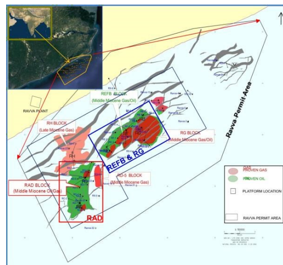
Figure 1: Location map of Ravva Field.
