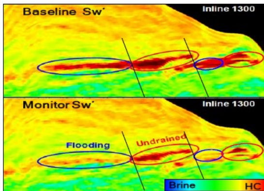
Figure 6: 4D saturation sections shows flooding signature and undrained areas
