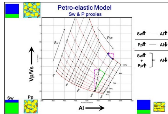
Figure 5: Petro-elastic Model (PEM) was generated using forward modeling.
