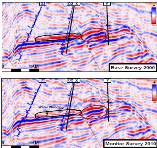
Figure 3: Far angle 4D seismic sections showing the movement of waterfront between 2000 & 2010.
