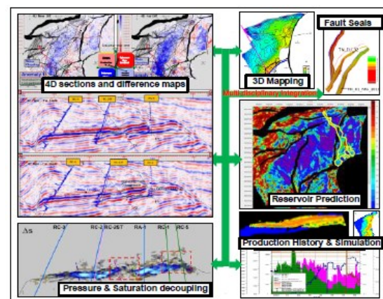
Figure 8: Integrated multi-disciplinary workflow
