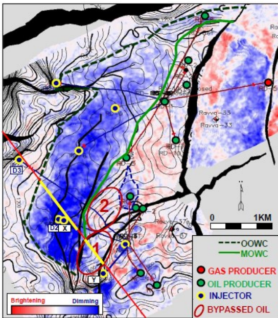
Figure 4: Sum of negatives map showing brightening (red) and dimming (blue).
