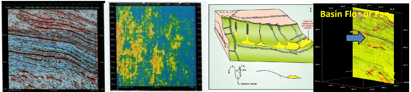
Fig.7a Trace XZ shows Basin floor fan Fig. 7b:Spectral slices at 24Hz Fig.7c : Eastern Basin floor fan schematic model & Voxel view
