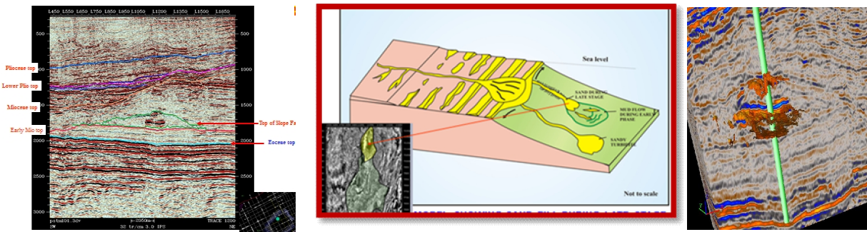
Fig: 4a Trace 1200 shows Slope fan Fig:4b Model of slope fan showing sand fill Fig.4c: Prospect I (Slope fan)-3D view (Later stage of forced regression)
