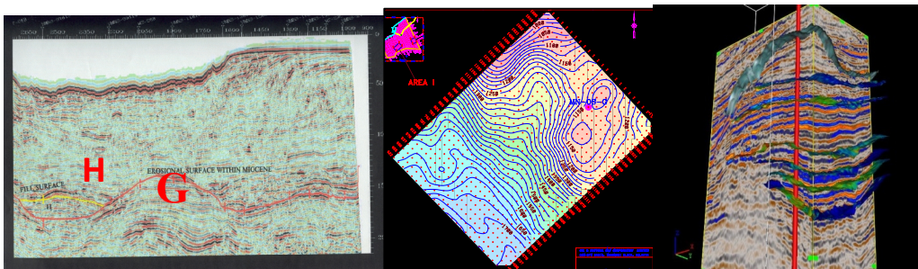
Fig:5a 2D line shows Relict feature G Fig:5b Structure map of Mio Pliocene Unconformity shows G Fig: 5c 3D view of Well XSW-1
