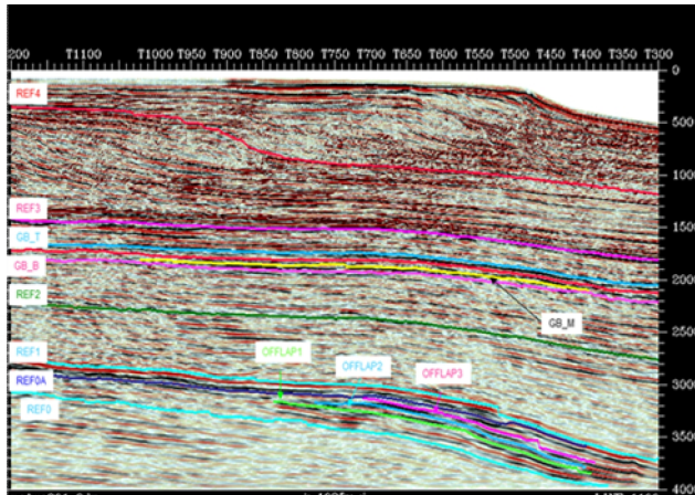
Fig.3 shows line XY of Study Area II showing mapped horizons
