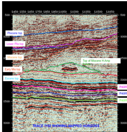
Fig.2 shows Trace XY of Study Area I showing mapped horizons
