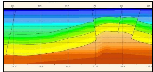
Figure 6: 2D Model for a seismic line across Atharamura Structure
