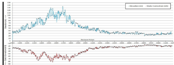
Figure 15: Static Correction Mirror image Plot
