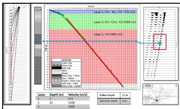
Figure 11: An interpreted uphole plot
