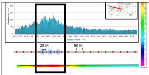
Figure 16: Closely spaced shots for the area of poor signal strength
