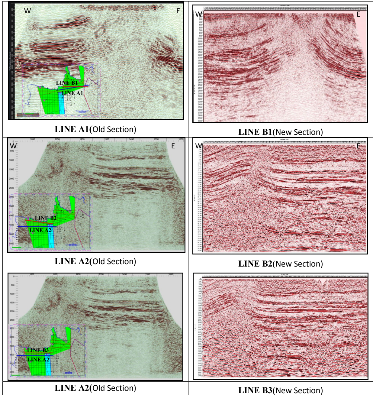
Figure 19: Comparison between seismic sections of earlier seismic investigation and the current one
