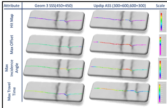
Figure 9: Comparison of different modeling attributes for conventional SSS and Up-dip flip flop ASS shooting
