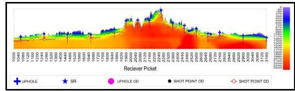
Figure 12: Near Surface Model of a seismic line across Atharamura Structure
