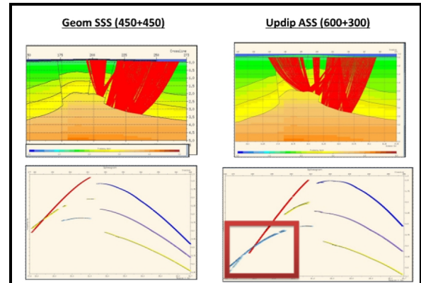
Figure 7: Comparison of Ray tracing Spikeogram between conventional SSS and Up-dip ASS shooting geometry
