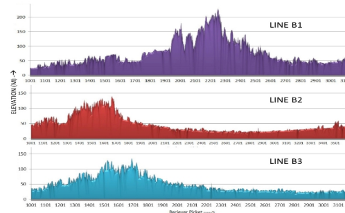
Figure 3: Elevation profile along the 2D seismic lines
