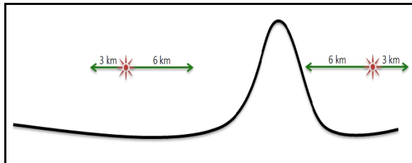
Figure 4: Flip-flip up-dip ASS Shooting Pattern
