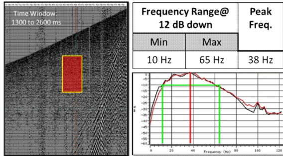
Figure 13: Frequency Spectrum Analysis
