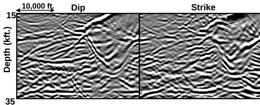
Figure 2. The imaging results for NAZ acquisition.
