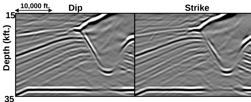
Figure 7. The imaging results for WAZ acquisition with no free surface multiples.
