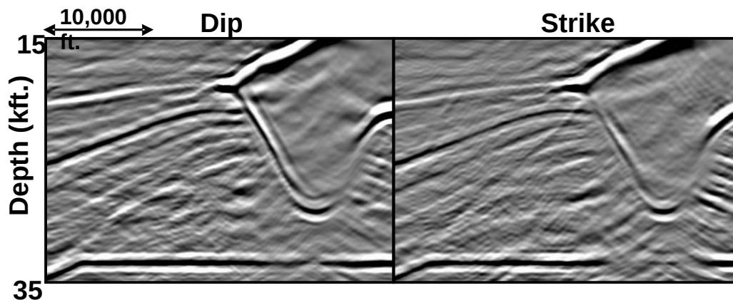
Figure 5. The imaging results for WAZ acquisition including 3D SRME.
