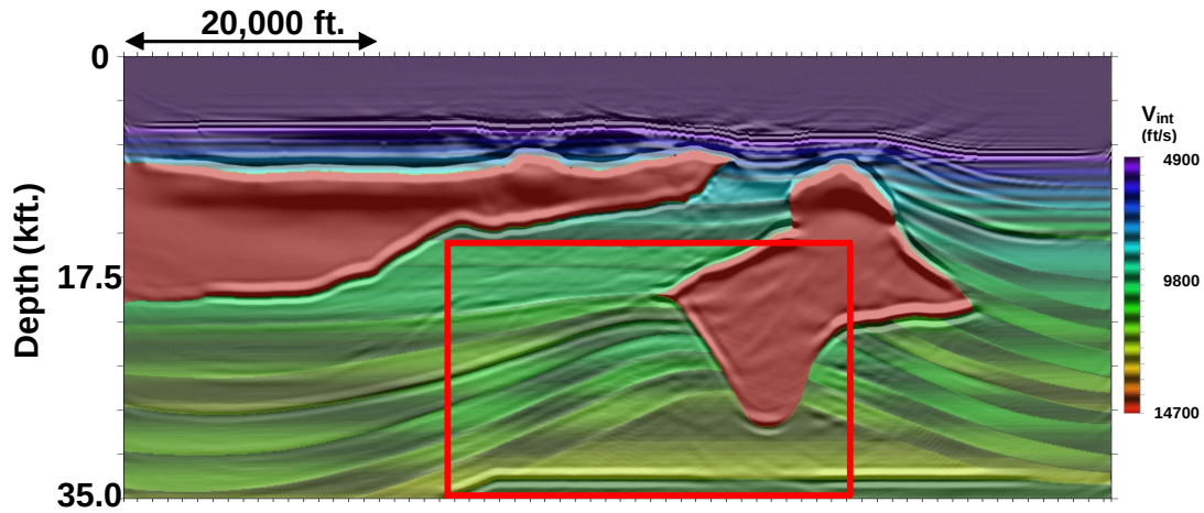
Figure 1. Velocity model for synthetic data. The red rectangle indicates the area shown in the subsequent displays.
