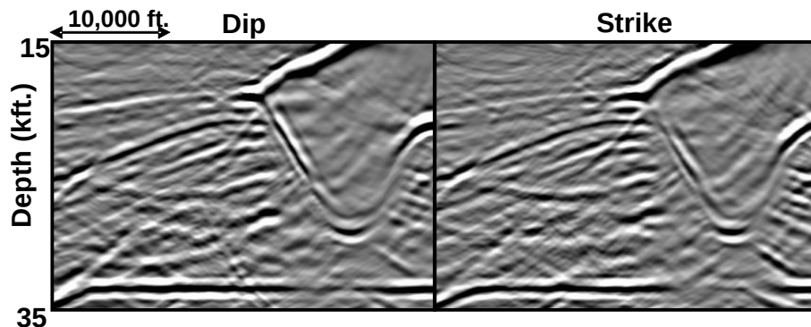
Figure 3. The imaging results for 4 km WAZ acquisition.
