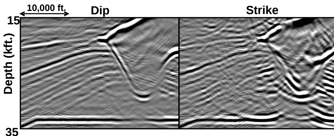
Figure 6. The imaging results for NAZ acquisition with no free surface multiples.
