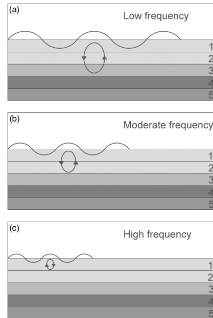
Fig. 1: a), b), and c) show simplified surface waves of a single frequency propagating along the surface of the earth, generated by three seismic sources with low, moderate, and high frequencies, respectively (figure courtesy of Olafsdottir (2014)). Each surface wave samples the subsurface at a different depth.
