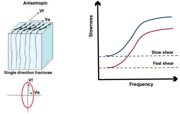
Fig. 3: Left side: Anisotropic model with a single set of fractures (top cube) and shear wave velocities as a function of direction (bottom red oval) (figure courtesy of Tinnin et al. (2008)). In anisotropic model with a single set of fractures, shear wave velocity is strongly anisotropic. Right side: As a result, the dispersion curves of two perpendicular directions (X and Y dipoles) shows significant separation.
