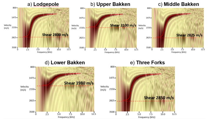
Fig. 5: a), b), c), d), and e) show the overlay dispersion images of the Lodgepole, Upper Bakken, Middle Bakken, Lower Bakken, and the underlying Three Forks, respectively. The solid lines indicate the main dispersion curves with highest amplitude in dark purple (they overlap in all studied formations). The dashed lines indicate low frequency dispersion tail approaching the formations shear velocity. The y-axis is in decreasing velocity (m/s) and the x-axis is in increasing frequency (kHz).
