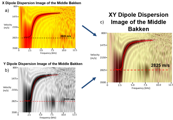
Fig. 4: a) shows X dipole dispersion image of the Middle Bakken in hot color map (highest amplitude in red), b) shows Y dipole dispersion image of the Middle Bakken in gray scale color map (highest amplitude in black), c) shows an overlay of X and Y dispersion images of the Middle Bakken with highest amplitude in dark purple. The solid lines indicate the main dispersion curves (overlap in this case) and the dashed lines indicate low frequency dispersion tail approaching the formations shear velocity. The y-axis is in decreasing velocity (m/s) and the x-axis is in increasing frequency (kHz).
