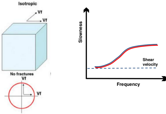
Fig. 2: Left side: Isotropic model (top cube) and shear wave velocities as a function of direction (bottom red oval) (figure courtesy of Tinnin et al. (2008)). In isotropic media with no fractures, shear wave velocity is azimuthally invariant. Right side: As a result, the dispersion curves of two perpendicular directions (X and Y dipoles) overlap.
