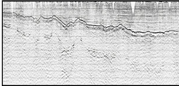
Figure 7: Static correction using first break pick time of the refracted wave.
