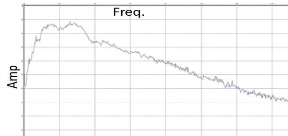
Figure 5: Amplitude spectrum for a single hole 20m, 5kg
