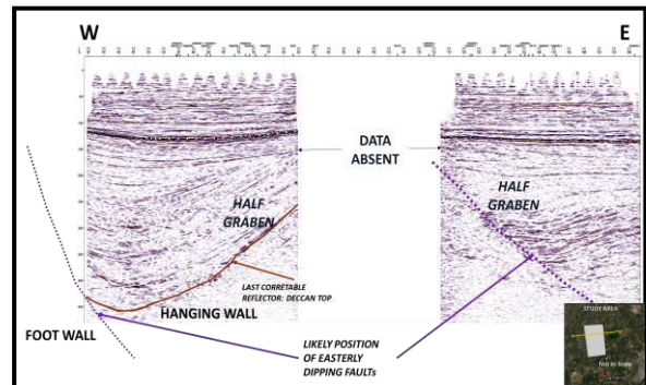
Figure.4b: EW section through northern part of study area depicting last correlative reflector and half graben geometry
