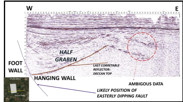
Figure.4a: EW section through southern part of study area depicting last correlative reflector and half graben geometry
