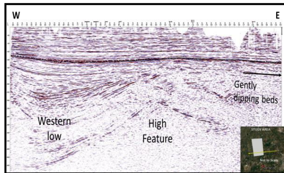
Figure.3: E-W section through Sanand High Structure
