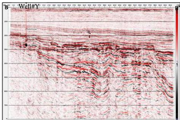
5.d Reprocessed PSDM Stack Section
