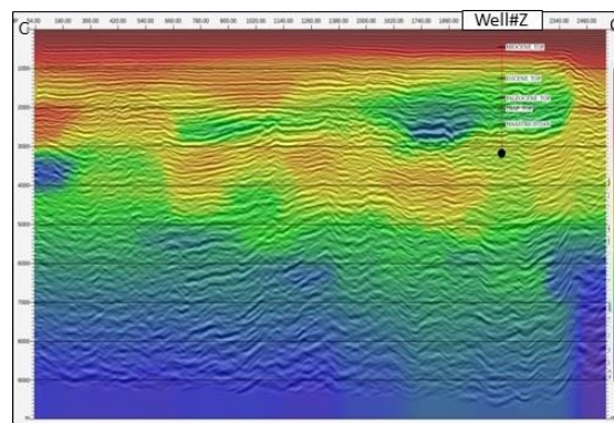
6.c Interval Velocity superposed on reprocessed PSDM Stack Section
