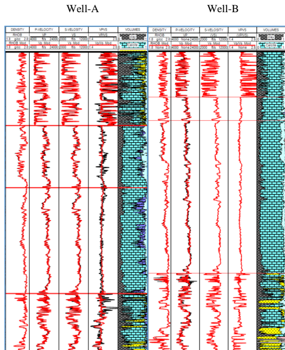
Figure 3: Petrophysical output of Well-A and Well-B along with P-velocity, Vp and S-Velocity, Vs. Recorded and predicted logs are shown in black and red respectively.
