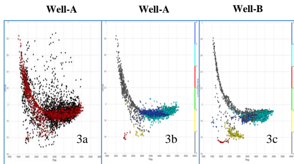
Figure (3a): Cross-plot generated between Pimp vs Vp/Vs ratio for recorded data of well-A. Figure (3b): Cross-plot generated between Pimp vs Vp/Vs ratio for modelled data of well-A. Figure (3c): Cross-plot generated between Pimp vs Vp/Vs ratio for predicted data in Well-B with Lithofacies
