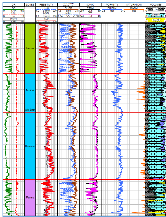
Figure 2: Petrophysical output of Well-A. Track 2 shows the lithology Clastic zone (in pink) has sandstone alongwith limestone and shale. Bassein and Mukta (in blue) zone is limestone and Heera (in green) is shale with limestone streaks.
