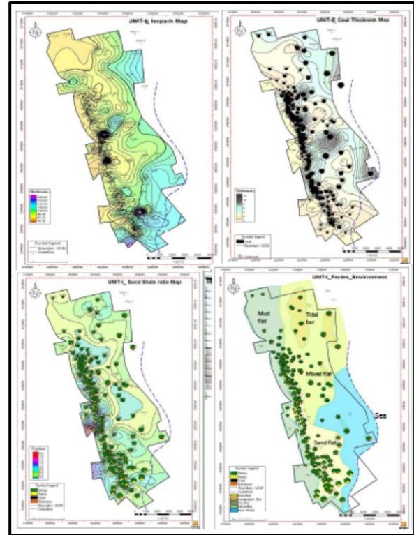
Fig-7: Isopach, coal thickness, sand/shale ratio maps and depositional environment of Unit-III
