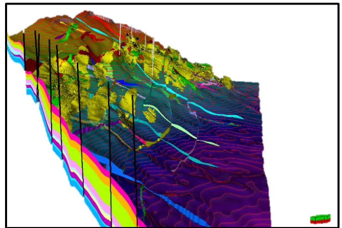
Fig-8: The 3D Geological Model of Mandhali Unit for the study area
