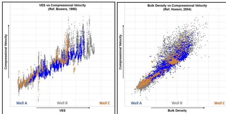
Fig 6: Bower's and Hoesni plots for Well A, Well B and Well C.
