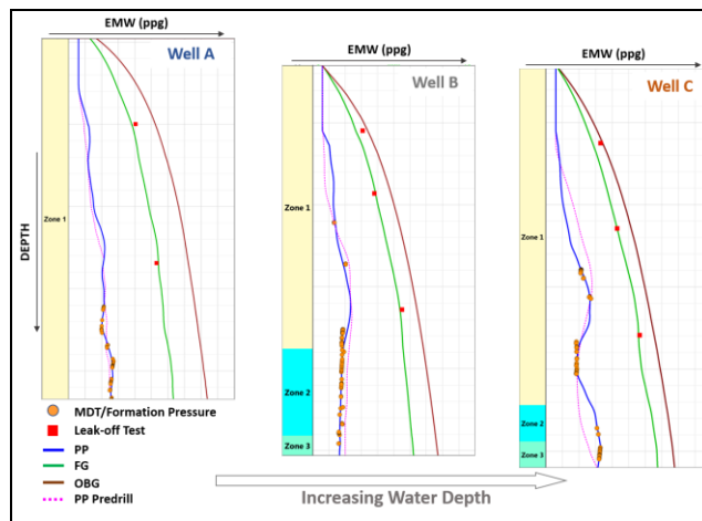
Fig 5: Post-drill pore pressure – fracture gradient models for the all three wells drilled till the time of this study.
