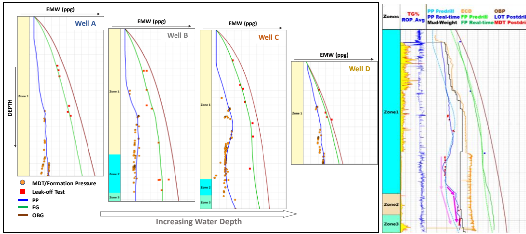
Fig 4(a): Pre-drill pore pressure and fracture gradient models for the four planned locations in increasing order of water depth; (b): Real-time pore pressure – fracture gradient monitoring window for Well C.
