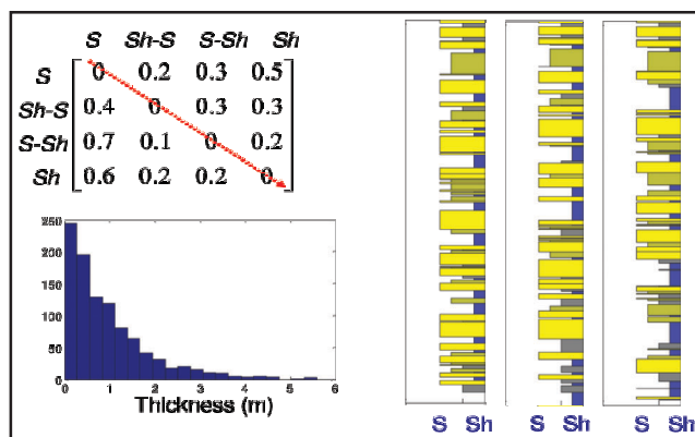
Fig.2 Examples of an embedded-form transition matrix with realizations of sequences. In this case, lithologic states are sand (s), shaly sand (sh-s), sandy shale (s-sh) and shale (sh). An example of thickness distributions used is shown in the lower left.
