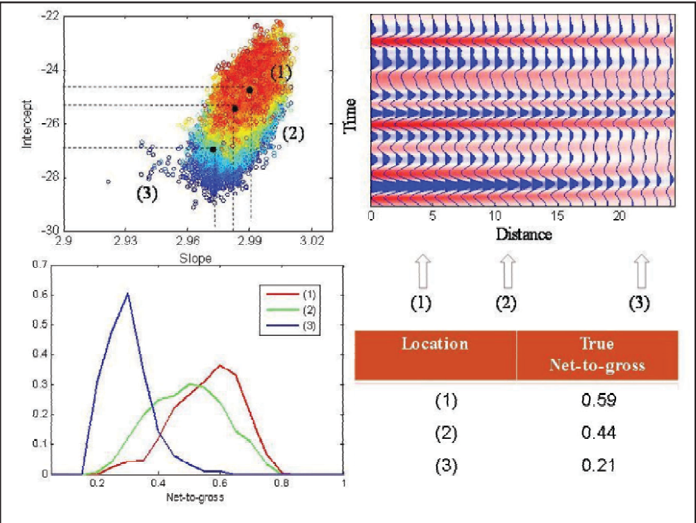
Fig.12 (Lower left corner) Posterior probability distributions of net-to-gross for three selected locations on the unknown seismic section labeled as (1), (2) and (3). The true values for each location are shown in the table at the lower right corner.
