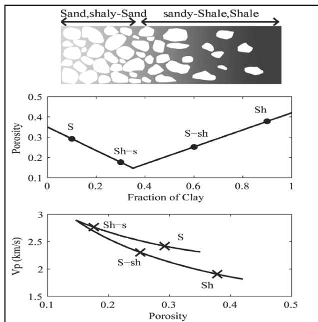
Fig.3 Illustrations of sand-shale mixtures, with their porosity and velocity values related to clay content (Modified after Marion, 1992). Porosity vs. clay content shows a V-shaped trend, where the two end points are the pure sand and pure shale porosity. Four lithologic states are marked including sand (s), shaly-sand (sh-s), sandy-shale (s-sh) and shale (sh).
