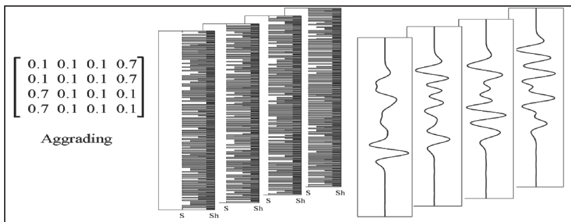
Fig.4 Examples of generated seismic response for multiple realizations of sequences.
