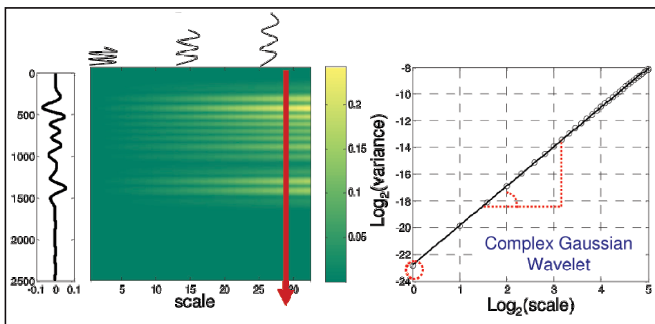
Fig.5 Example plot of wavelet transform of a seismogram (left) and plot of log (scale) versus log (variance of modulus of wavelettransform coefficients) and the linear fitting curve.
