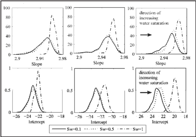
Fig.9 Distributions of slope and intercept values corresponding to the 3 transition matrices in Figure 8 in the same order from left to right.
