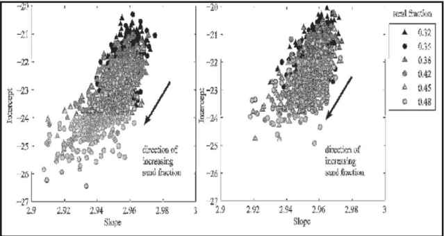
Fig.6 Plot of slope and intercept of wavelet transforms of seismic responses for 2 different standard deviations of velocities: (Left) 0.1 km/s and (Right) 0.2 km/s. Points correspond to sets of 200 Monte Carlo simulations generated from different transition matrices with various sand fractions (sand). Sw is 0.1 for sand layers and 1 for the others.
