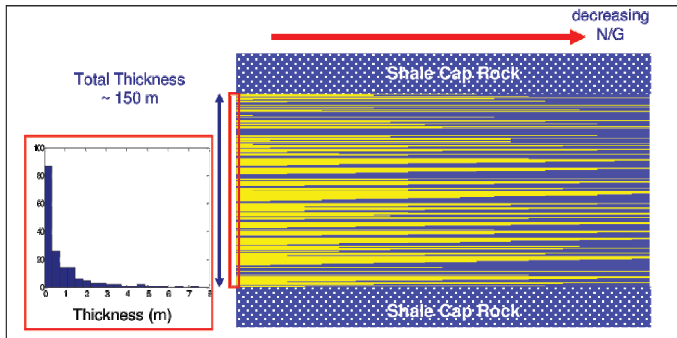
Fig.10 A realization of 2-D geologic section used in the numerical example. The area at the left end marked with the red box corresponds to the well location. Sand and shale are colored in yellow and blue respectively. The thicknesses of sand layers decrease linearly away from the well. The total thickness of reservoir is 150 m. An example of the thickness distribution used to simulate the sequence at the well location is also shown.
