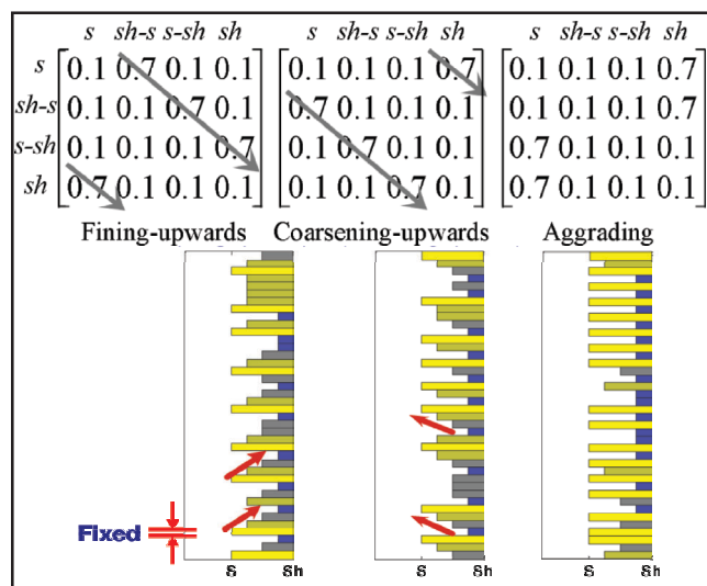
Fig.1 Examples of transition matrices with fixed sampling intervals. Three different types of geology are shown: fining upwards, coarsening upwards, and aggrading sequences. In this case, lithologic states are sand (s), shaly sand (sh-s), sandy shale (s-sh) and shale (sh). The off diagonal elements marked by arrows control the directionality of the sequences.
