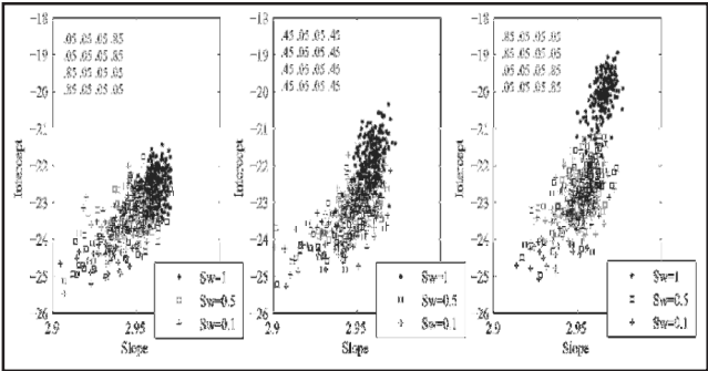
Fig.8 Plot of slope and intercept of wavelet transforms of seismic response for sequences generated by 3 different transition matrices. All matrices have a similar limiting distribution: [0.45 \ 0.05 \ 0.05 \ 0.45] . Different values of water saturation in the sand layers (i.e. Sw=0.1, 0.5 and 1 ) are shown in the legend.
