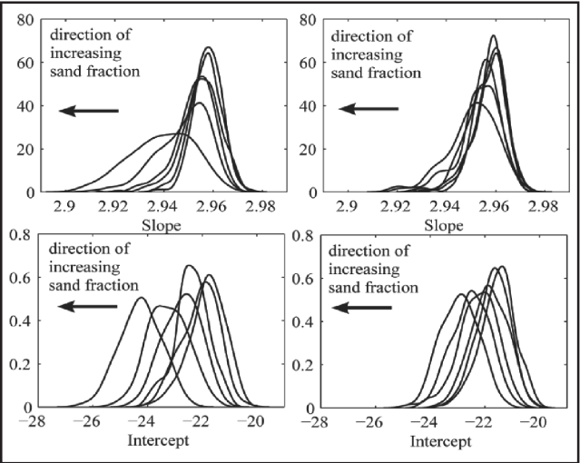
Fig.7 Probability distributions of slope and intercept values corresponding to data points in Figure 6 for both values of standard deviations. The direction of increasing sand fractions (sand) is to the left for all plots.
