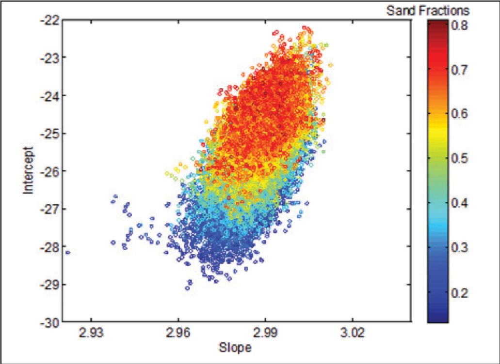
Fig.11 Results of 1000 realizations of 2-D sections show how slope and intercept vary with varying sand fractions.
