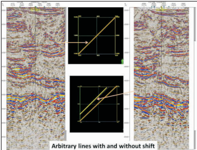
Fig. 10: Arbitrary lines with and without shift
