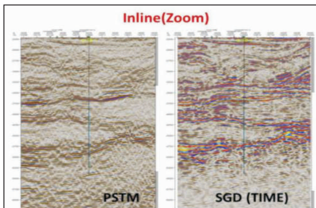
Fig. 1: Comparison between initial PSTM and SGD Baseline processed section.
