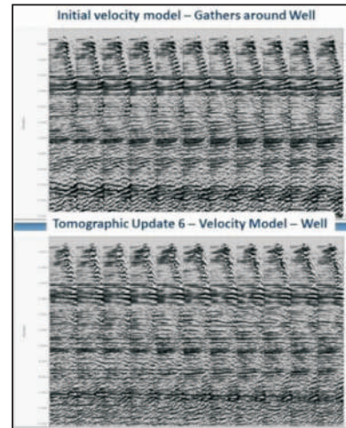
Fig. 5a: Initial and final velocity model : gather updates
