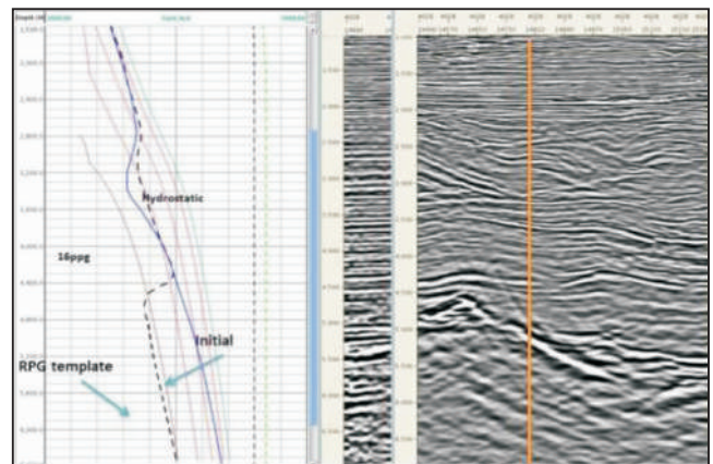
Fig. 6: Velocity, Gather, Stack at well location:Initial
