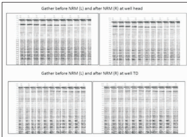
Fig. 3: Gathers before and after NRM at well head and TD
