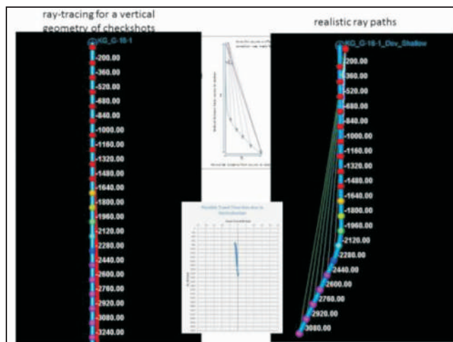
Fig. 2: Corrections for raypaths even smaller in magnitude, were applied to maintain accuracy in imaging.
