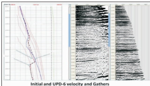
Fig. 4: Initial and final velocity and gathers display.
