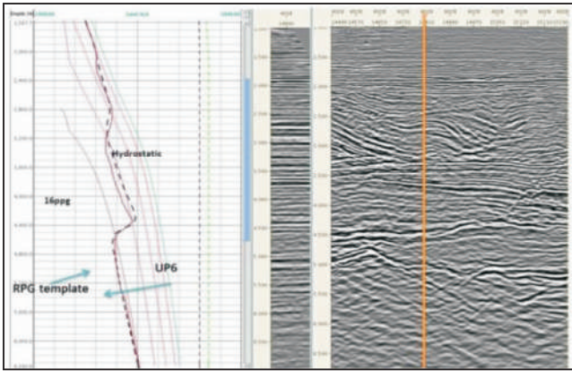
Fig. 8: Velocity, Gather, Stack at well location: Update-6
