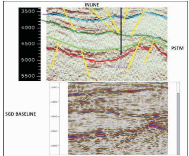
Fig. 11: Seismic section PSTM and SGD baseline
