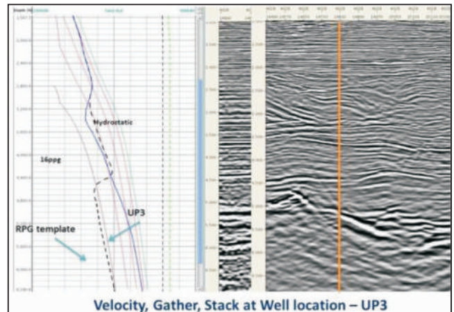
Fig. 7: Velocity, Gather, Stack at well location: Update-3
