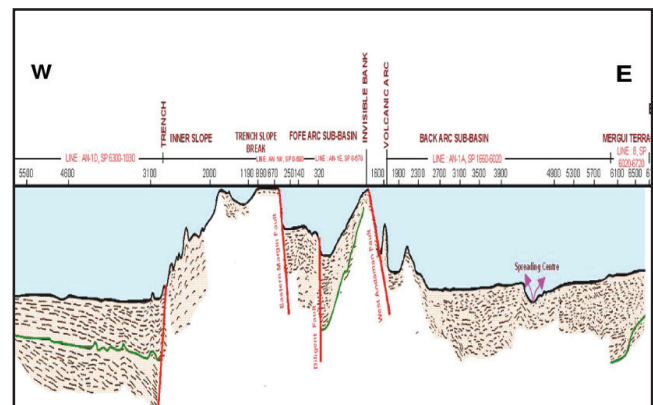
Fig. 3: A Geological Section across the Andaman-Nicobar Basin (E-W direction)(Source: DGH website)
