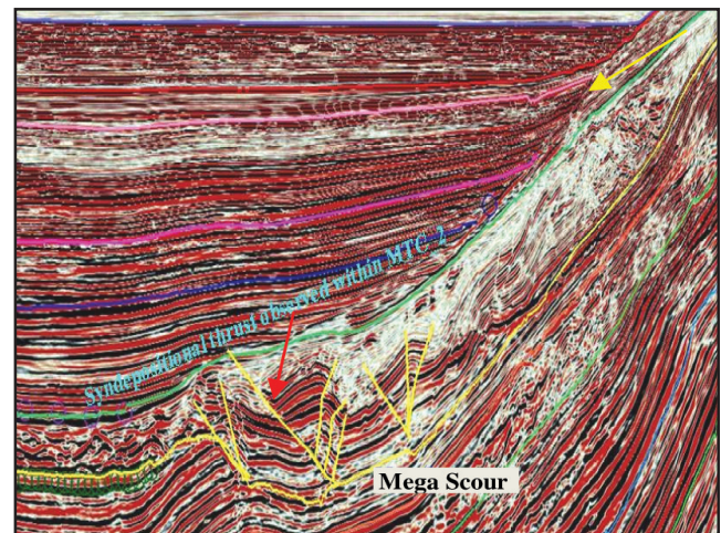
Fig. 7: The slump, part of the MTC shows compressive syndepositional thrust feature and mega scour at the bottom.
