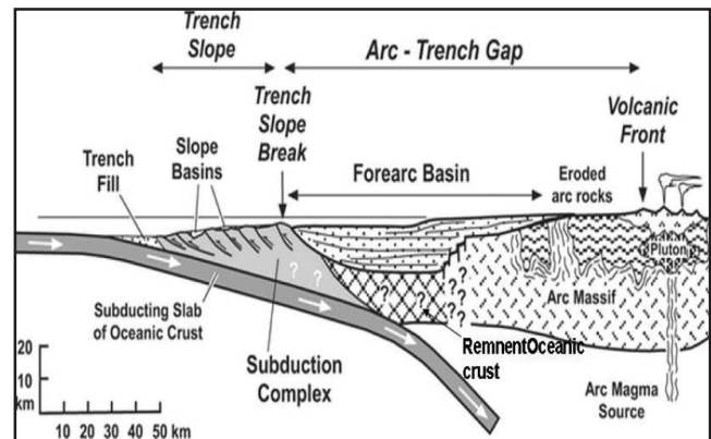
Fig. 2: Generalized Forearc model.
