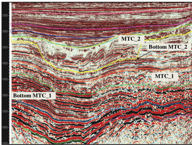
Fig. 4: N-S seismic line showing presence of two big MTC sequence within the study area separated by finer clastics deposit.
