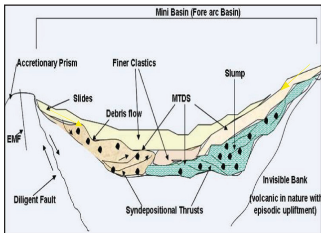
Fig. 8: Conceptual model for deposition of MTCs in deep water of Andaman Forearc Basin. The model indicates a detached MTC whose genesis is associated with over steepening of one of the margin of the mini basin.
