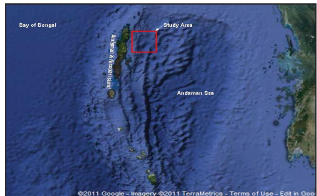
Fig. 1: Location map and area of study in Andaman-Nicobar Island (from Google Maps).
