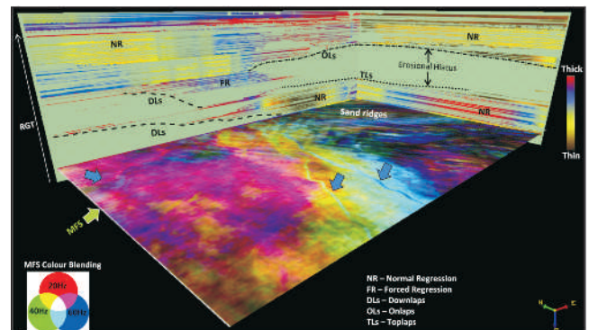
Fig.4: An illustration for 4D Wheeler Diagram allowing a comprehensive investigation of depositional environments in space and their development through geologic time. The systems tracts isochron attribute display on sections (or volume) helps define a unit completely (space-time). The horizontal slice (colour blended spectral decomposition responses) represents a particular depositional surface (maximum flooding surface) along which detailed patterns are enlightened.
